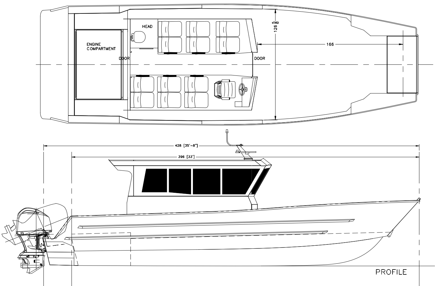
Base Platform Layout
