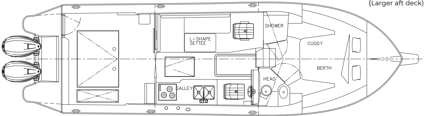
Layout Option A (Quarter Berth)
