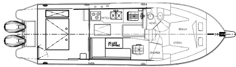
Base Platform Layout (Larger aft deck)
